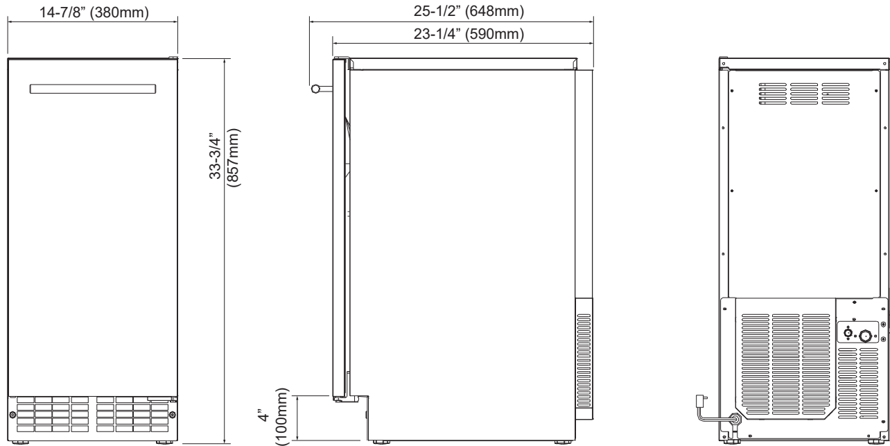
OVER ALL DEPTH WITH DOOR @ 90° - 37-1/4"
