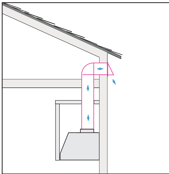
WALL EXHAUST
