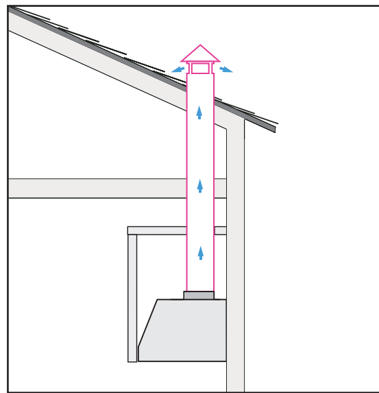
ROOF EXHAUST
