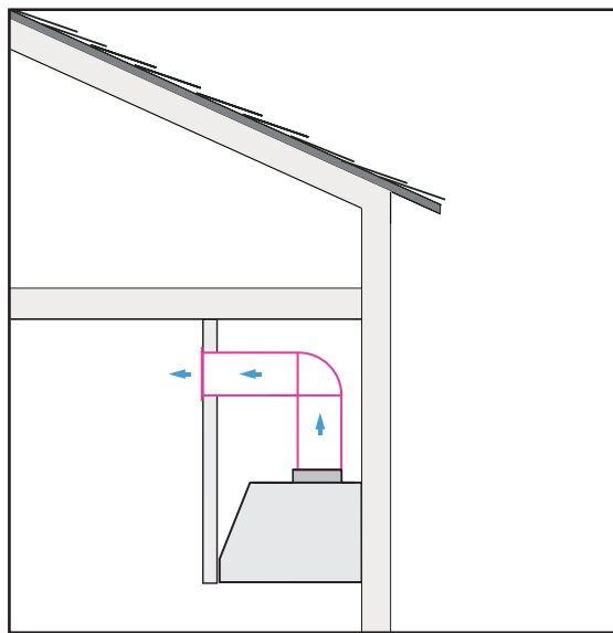
SOFFIT EXHAUST
