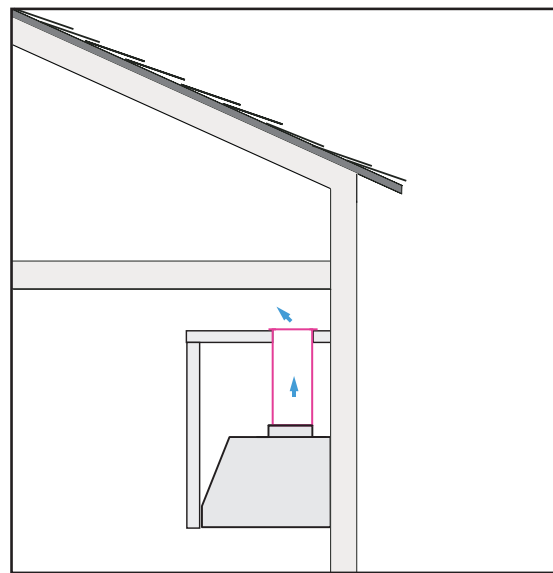
CABINET TOP EXHAUST
